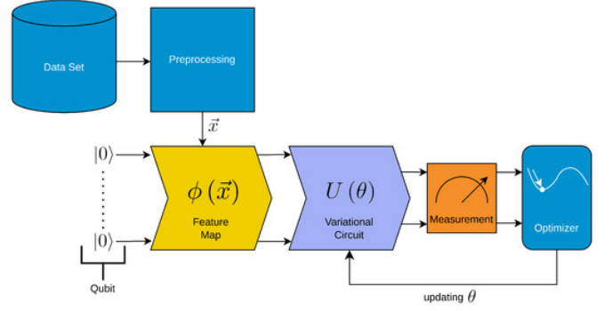
Fig. 6. Illustration of the application of quantum computing for manipulating data sets [28]. We can visually see here the usage of optimization techniques and programming for a desired output, dependant on the algorithm.
