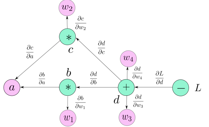
Fig. 5. Illustration of tensor networks through backpropagation to minimize a loss function [21]. The transaction channels can be represented by multiple tensors that can split off respectively depending on intended algorithms that is widely applicable in machine learning. We can also visually see the backpointing technique in storing checkpoints. Our single \alpha tensor network serves as a fundamental representation in equation (15).
