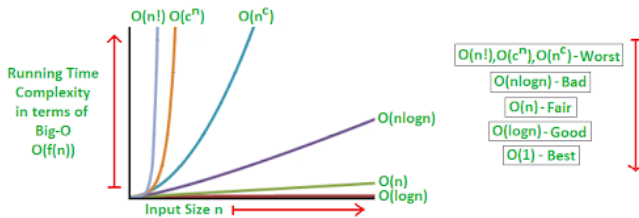
Fig. 3. Examples of Big-O complexities [15]. Our goal is finding a low computational cost towards the bottom of the graph.
