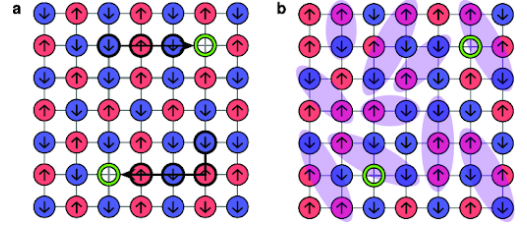
Fig. 2. Illustration of 2-D cartoon quantum tunneling of Hubbard fermions [10].
