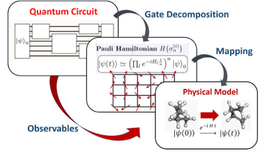
Fig. 4. Illustration of state preparation and mapping of models with the intermediate step of transformation [16].
